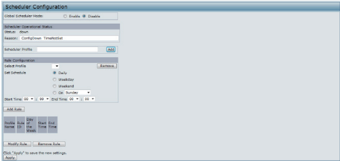
Figure 19 - Scheduler Configuration
