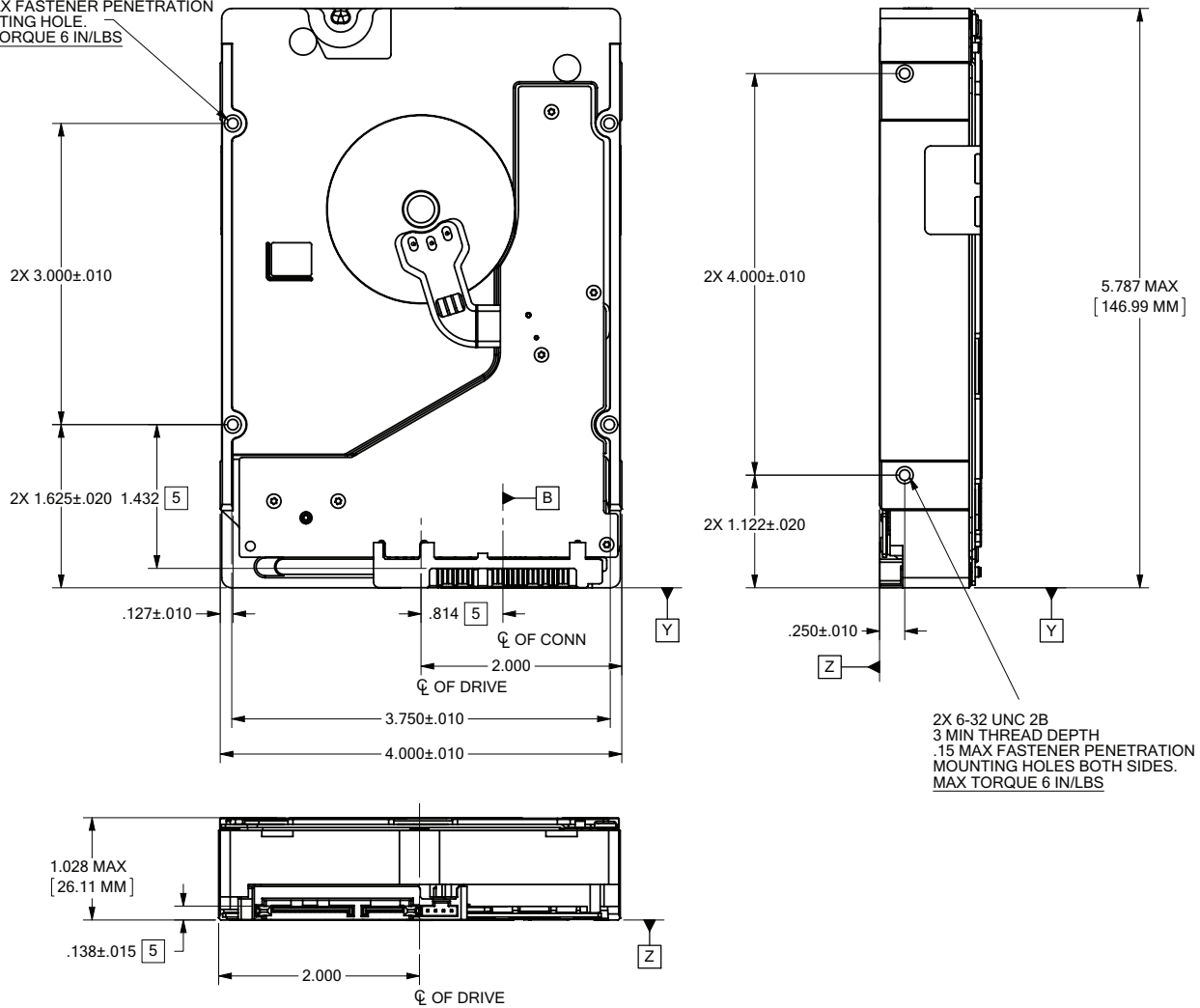
Figure 4. Mounting configuration dimensions (10TB and 8TB models)
