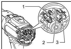
1. Arm 2. Spring 3. Recessed part
