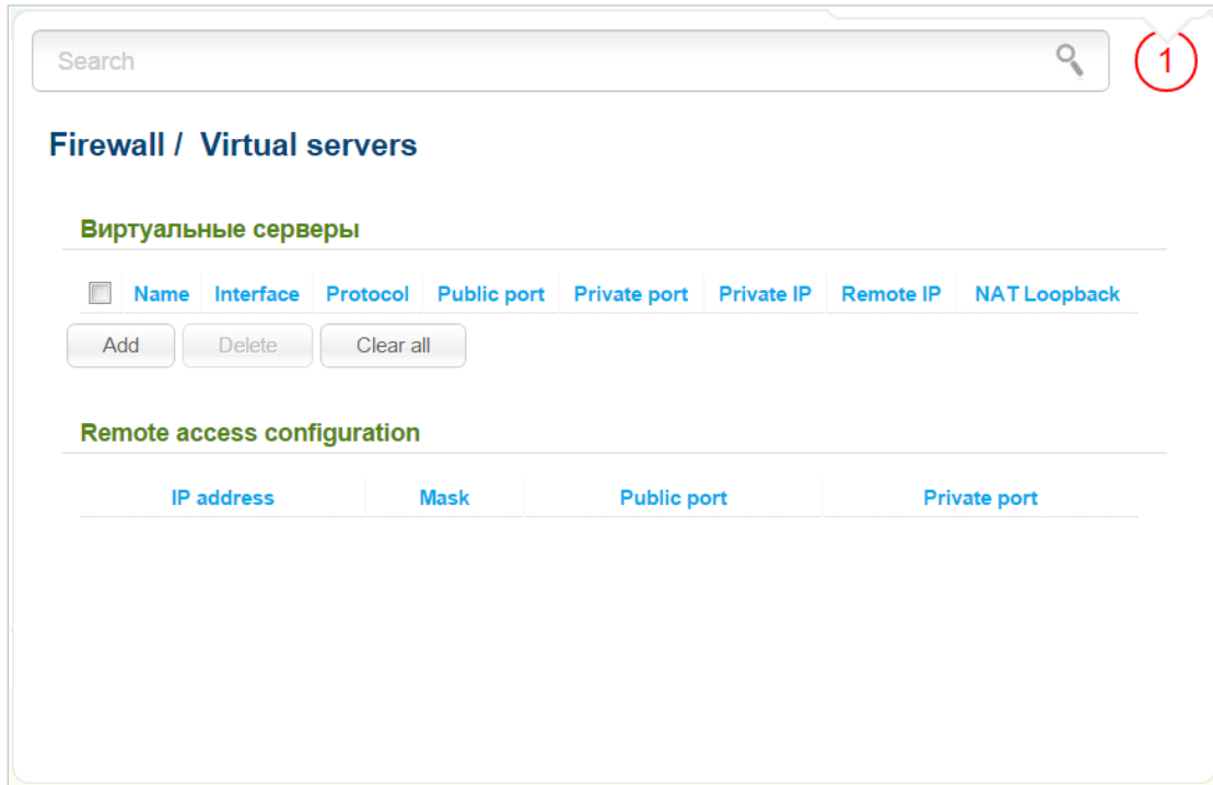
Figure 122. The Firewall / Virtual servers page.
