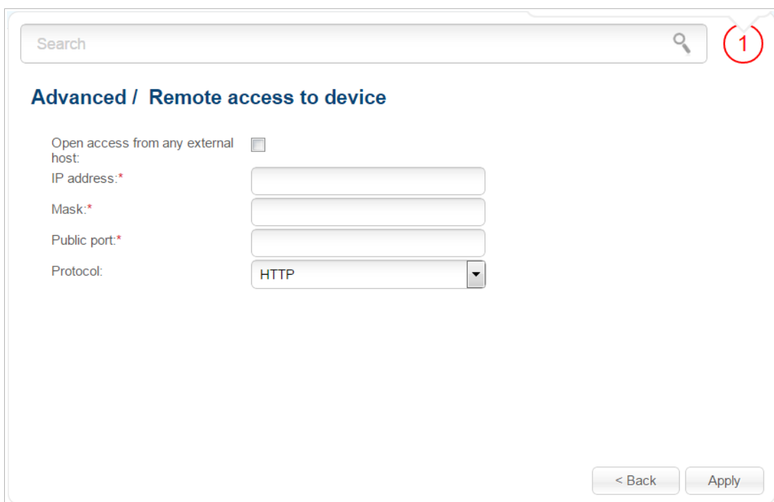
Figure 116. The page for adding a rule for remote management.
