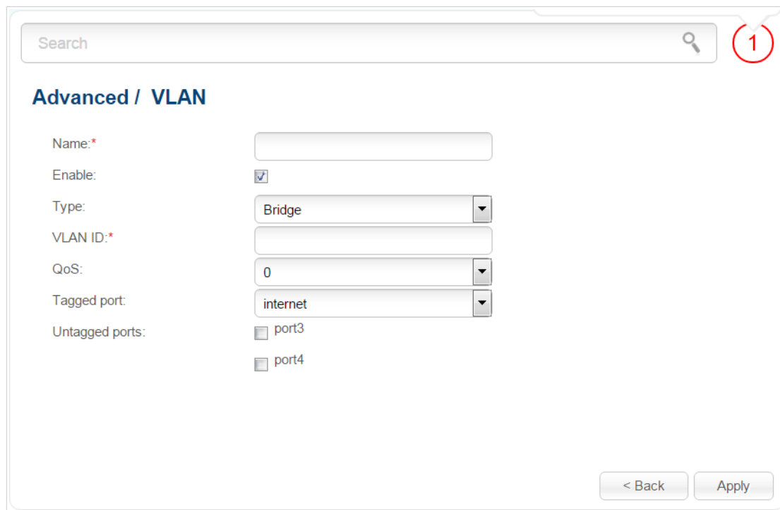
Figure 109. The page for adding a group of ports for VLAN.
