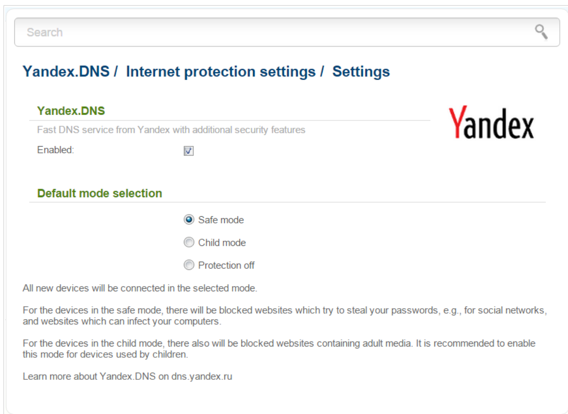
Figure 129. The Yandex.DNS / Internet protection settings / Settings page.
