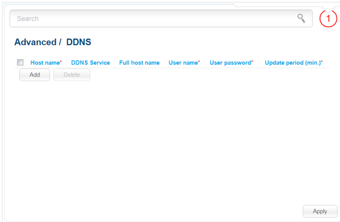
Figure 112. The Advanced / DDNS page.
