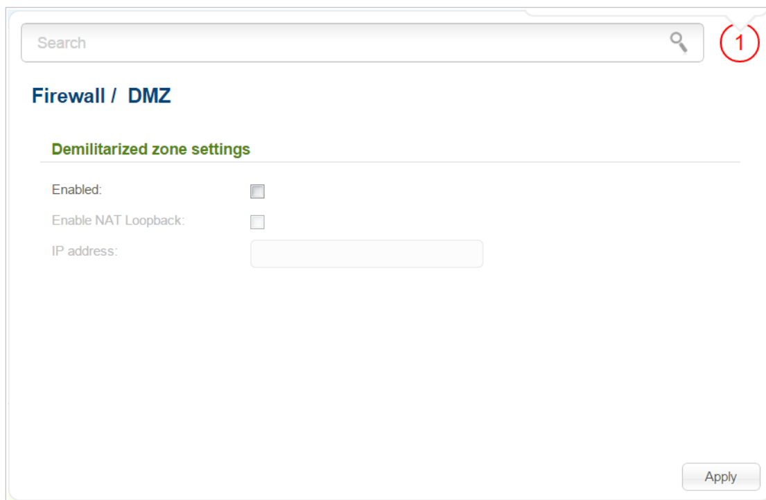
Figure 124. The Firewall / DMZ page.
