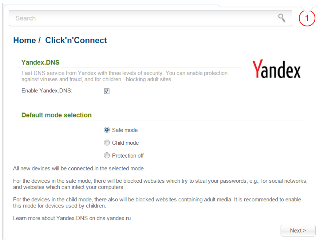
Figure 42. Configuring the Yandex.DNS service.
