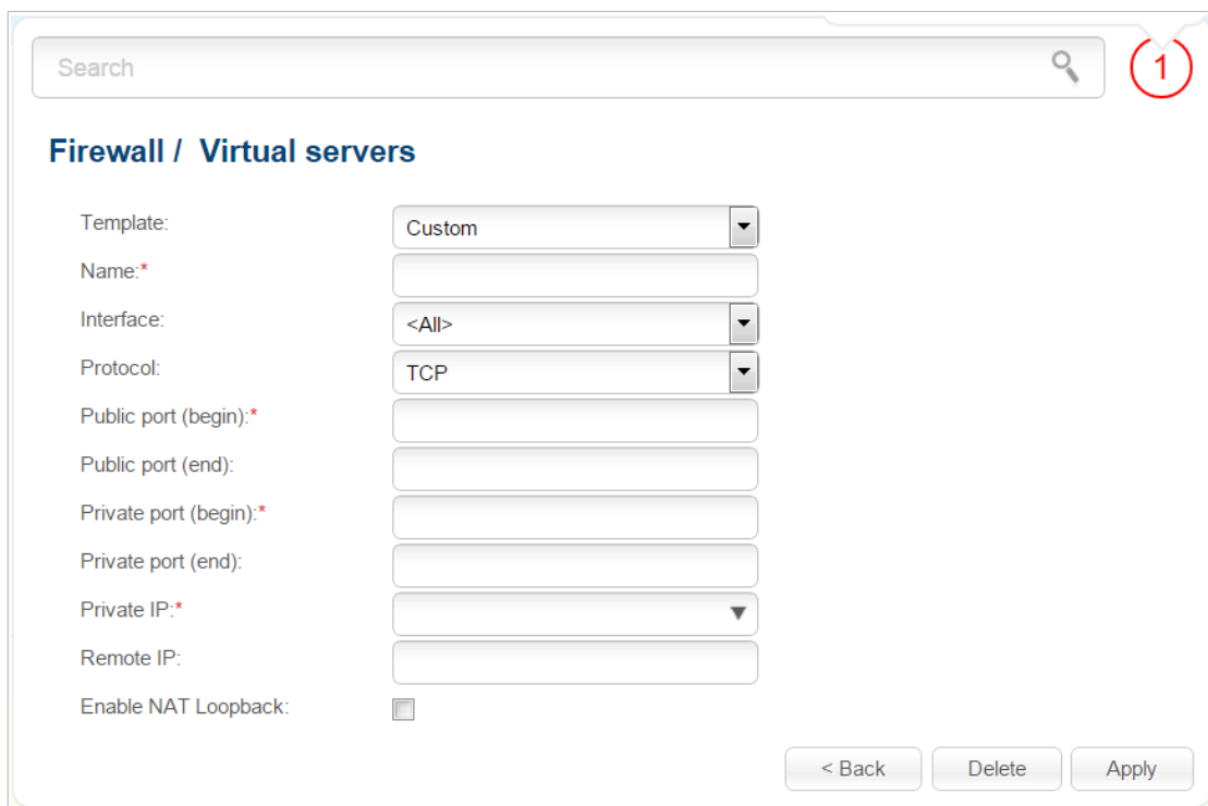
Figure 123. The page for adding a virtual server.
