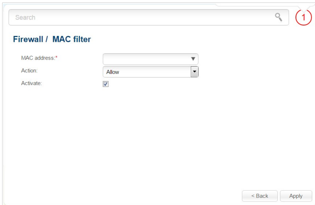
Figure 126. The page for adding a rule for the MAC filter.
