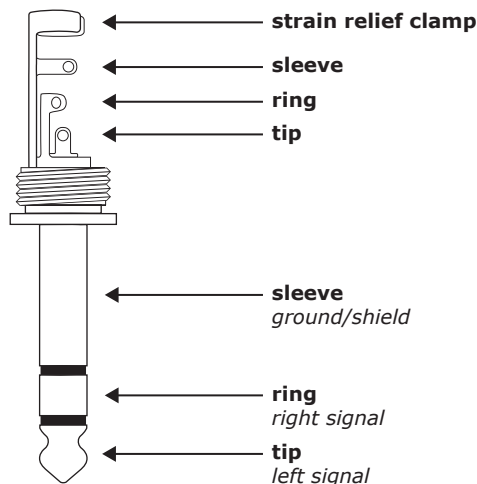
Fig. 3.3: 1/4" TRS connector
