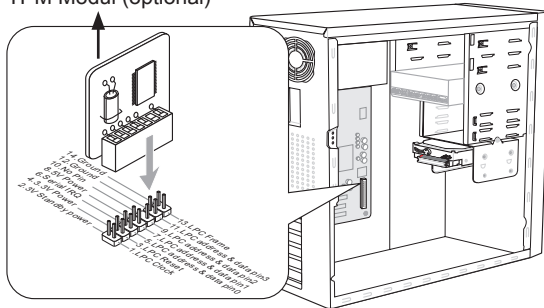
TPM Modul (optional)
