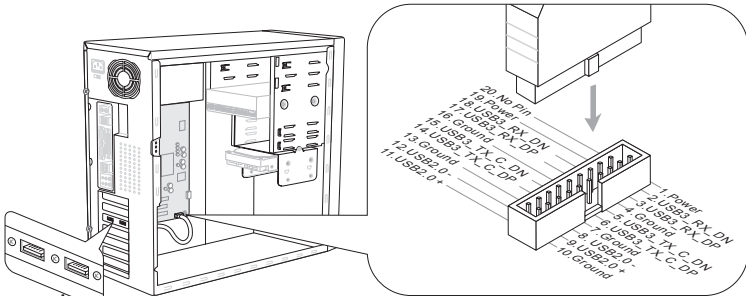
USB 3.0 Bracket (optional)
